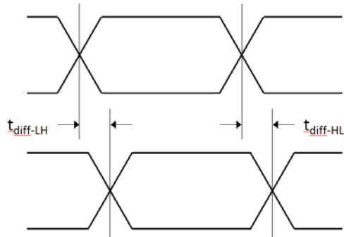
Figure 10. Propagation Delay
