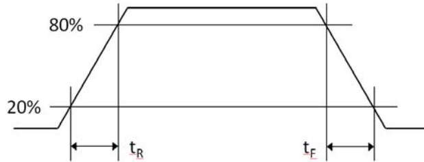
Figure 11. Output Rise and Fall Times
